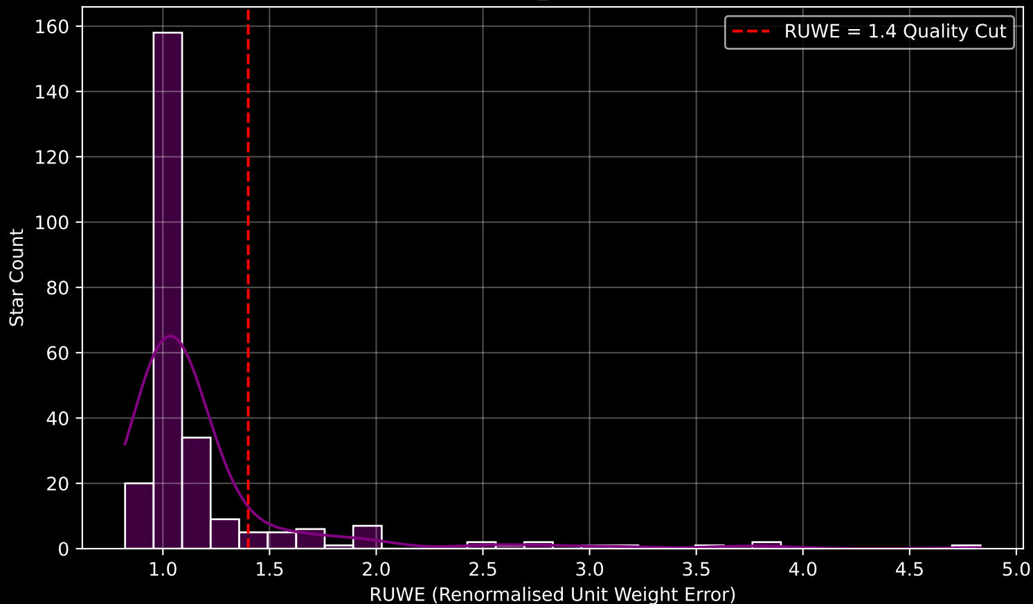
GAPOGEE DR17 Field [024+64_btx] RUWE Distribution (n= 256)
