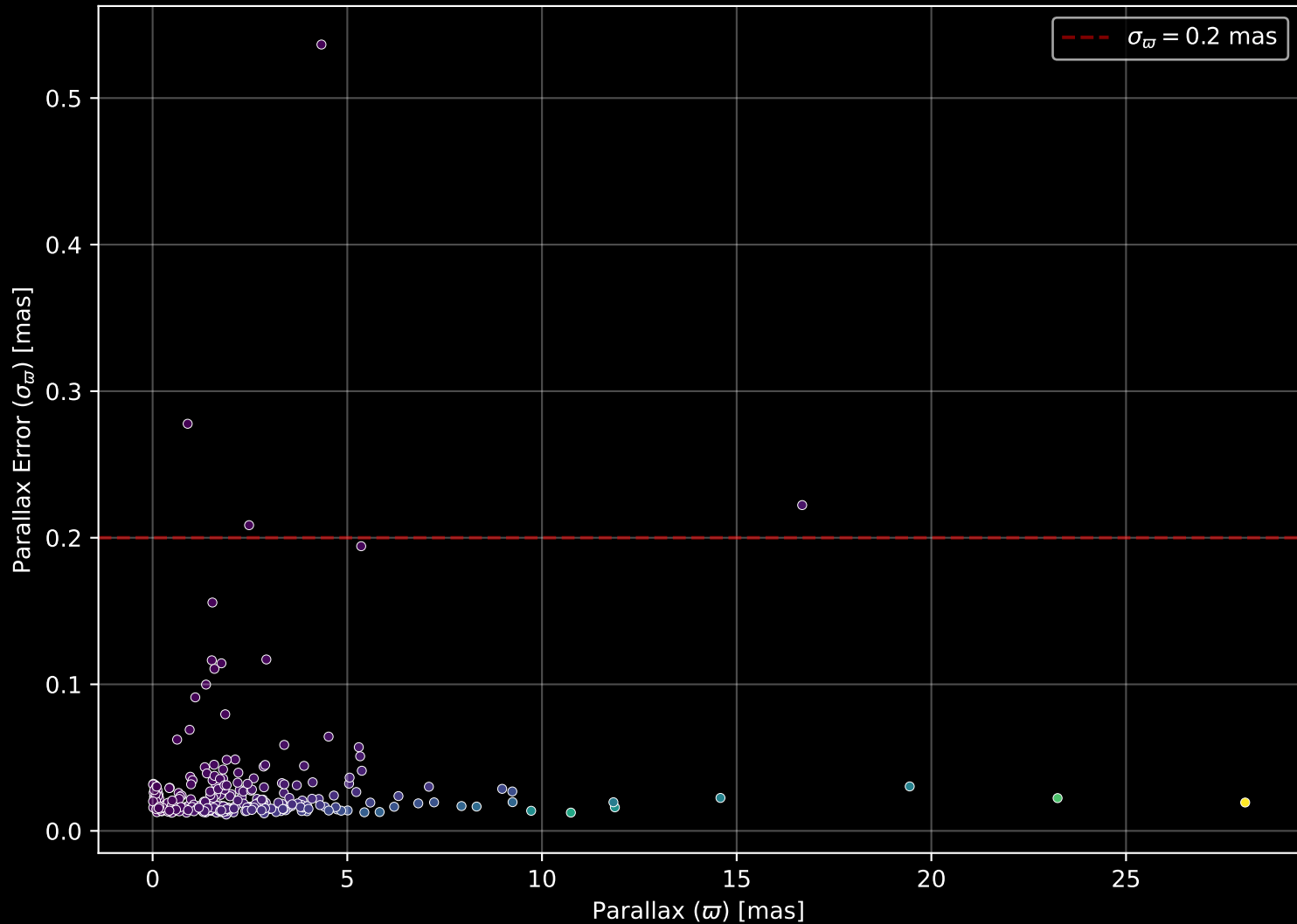
APOGEE DR17 Field: [024+64_btx] Parallax Quality (n= 265)
