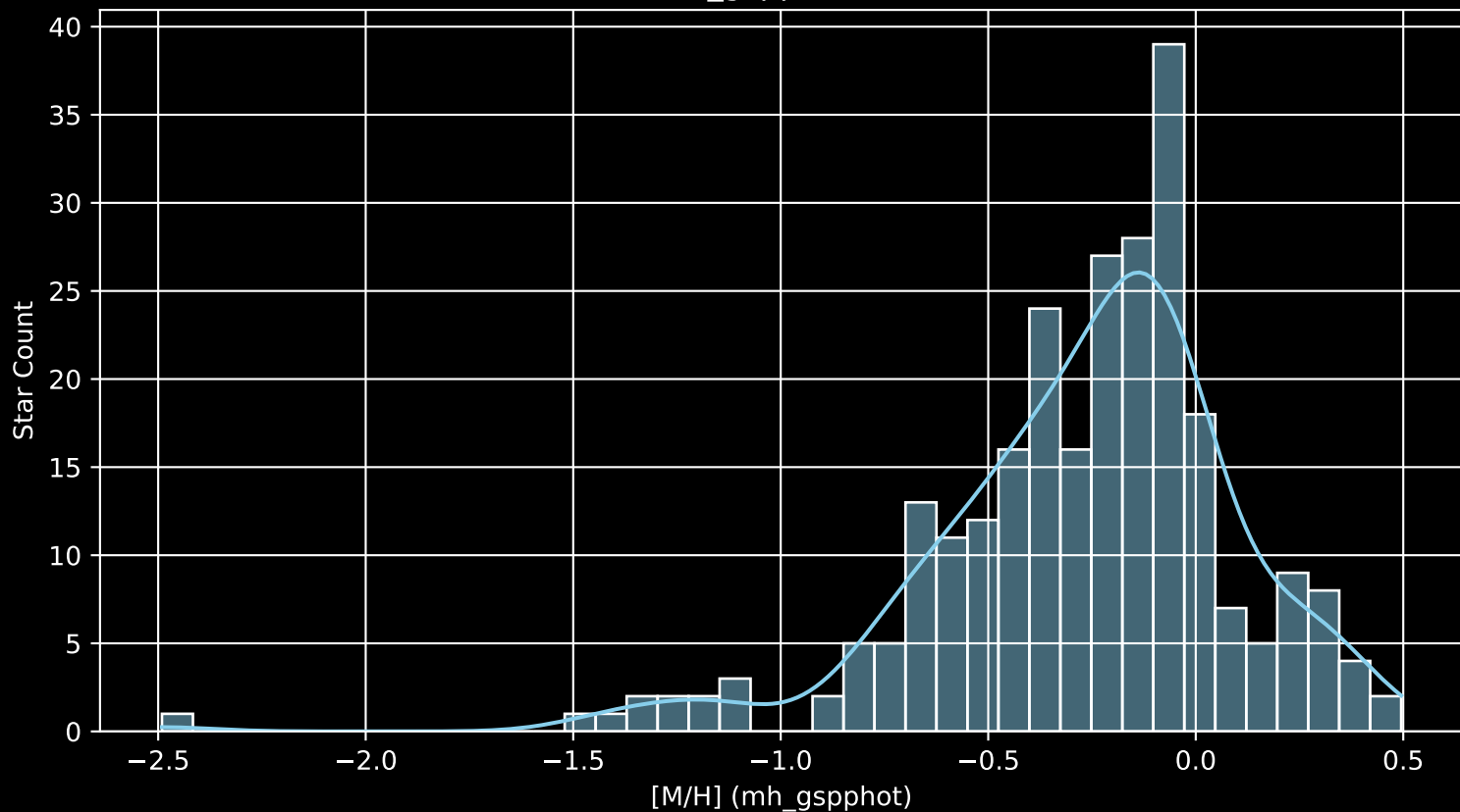
APOGEE DR17 Field: [024+64_btx [M/H] (mh_gspphot) (n= 263)
