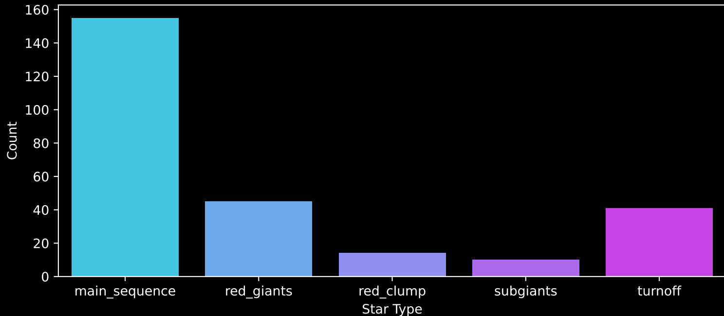
APOGEE DR17 Field: [024+64_btx] Count plot of Star Type
