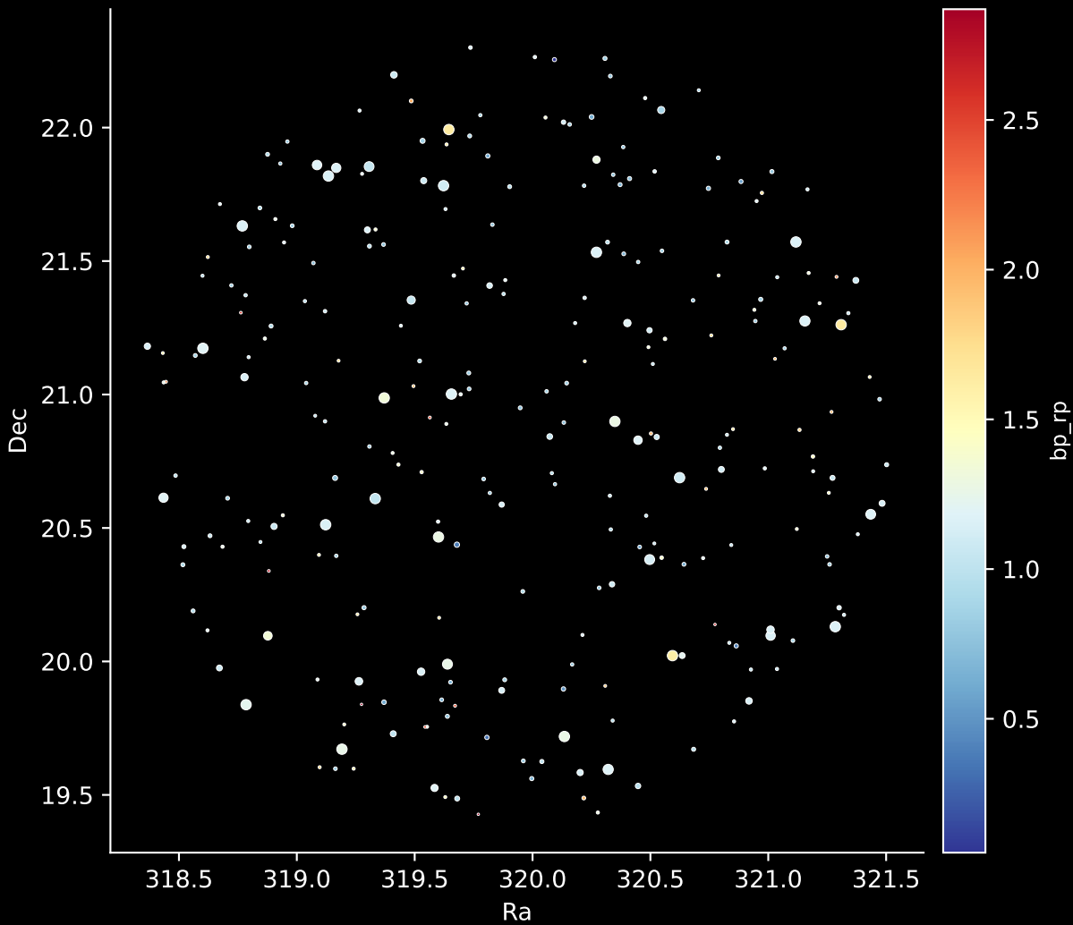
APOGEE DR17 Field: [024+64_btx] Stars: 265
