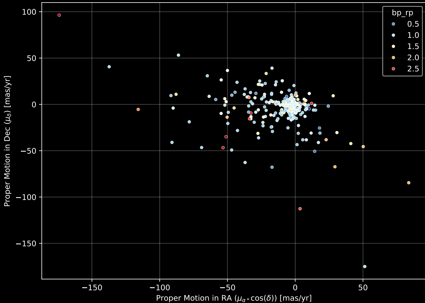
APOGEE DR17 Field: [024+64_btx] Proper Motion Diagram (n= 265)
