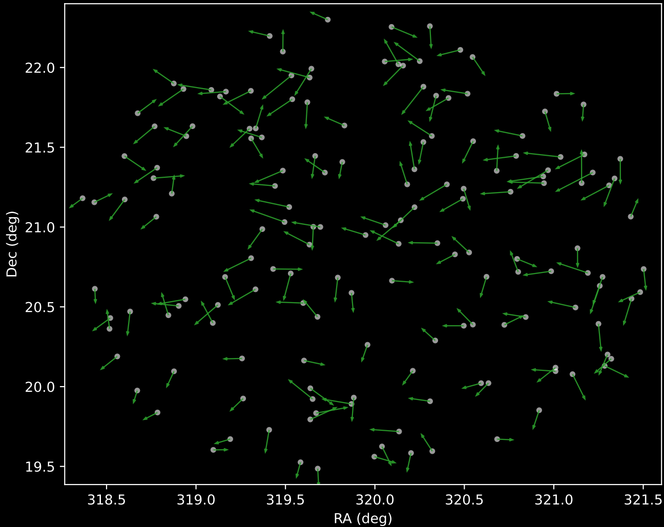
APOGEE DR17 Cluster 4 Proper Motion Vectors (n=161)
